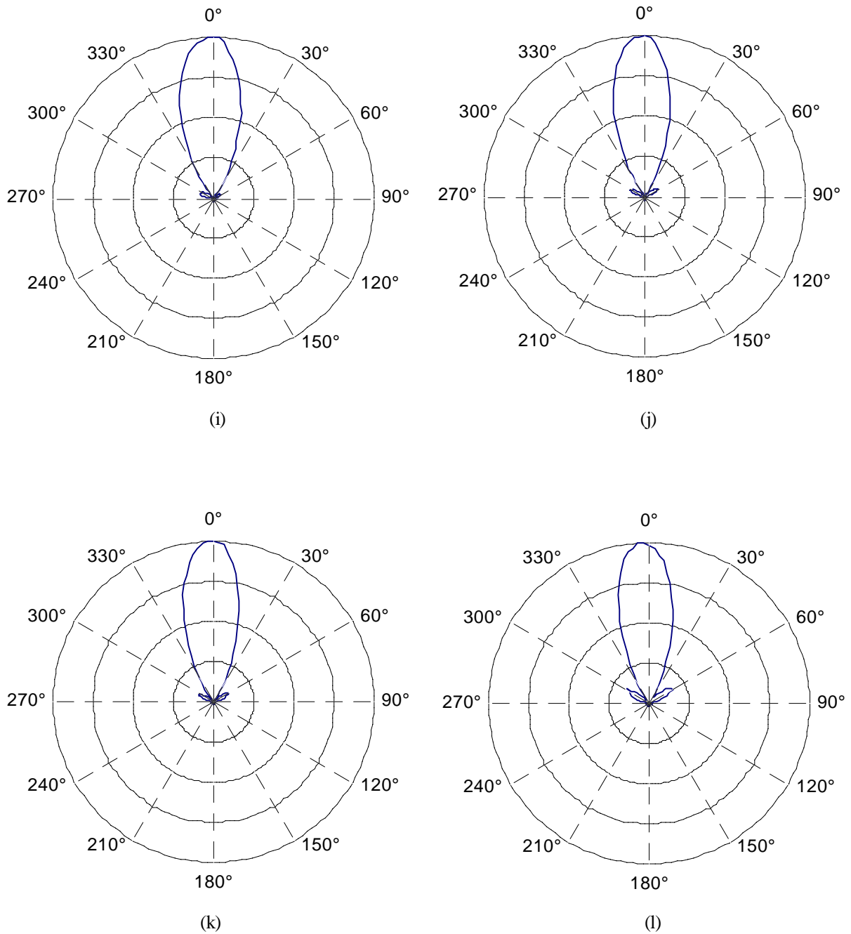
Figure 5.1 Measured power patterns for the representative case at (i) 1.9 GHz, (j) 1.95 GHz, (k) 2.0 GHz, and (l) 2.05 GHz.
